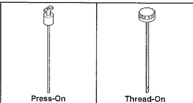
Figure 6. Dipstick Styles.
