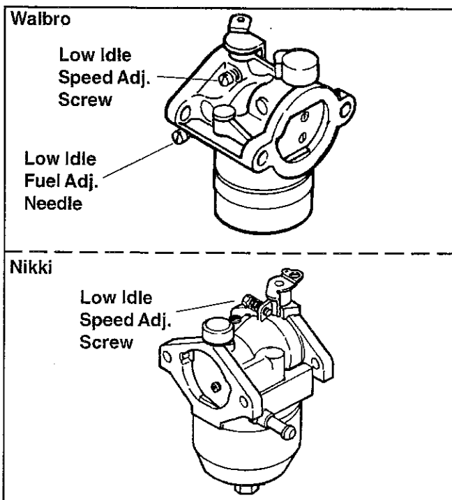
Figure 13. Carburetors.
